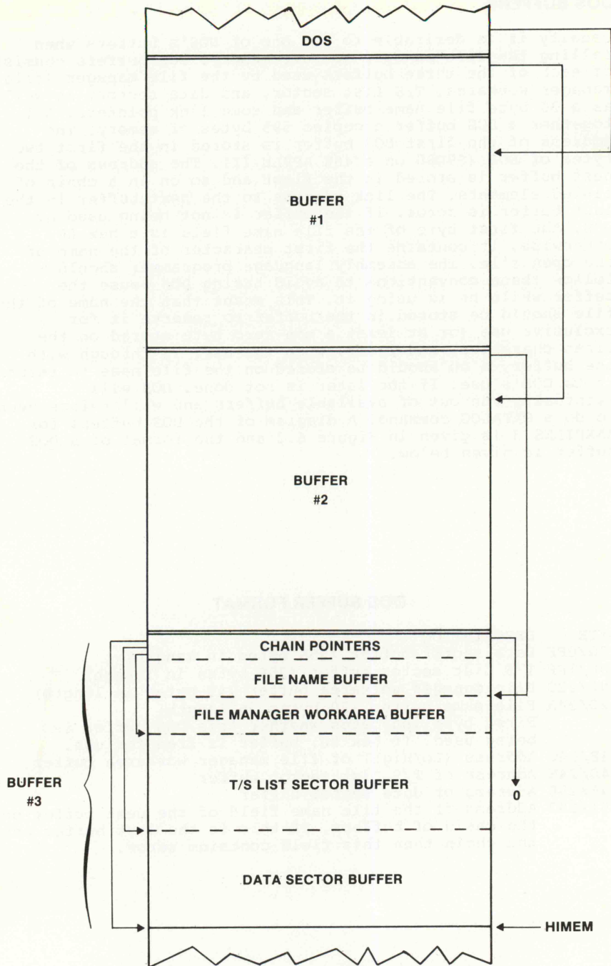
FIGURE 6.3 — DOS FILE BUFFERS
