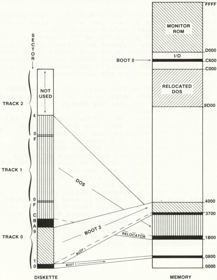
FIGURE 5.2 - BOOTSTRAP PROCESS
